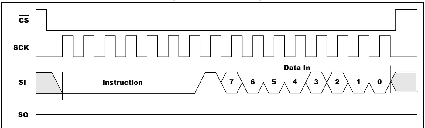
Figure 5-5. WRSR Timing
