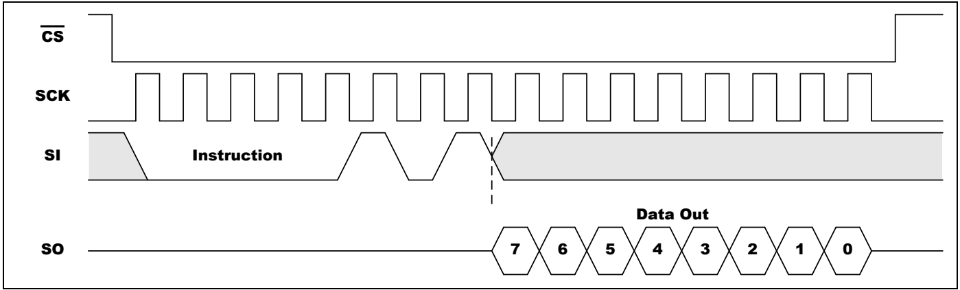
Figure 5-4. RDSR Timing
