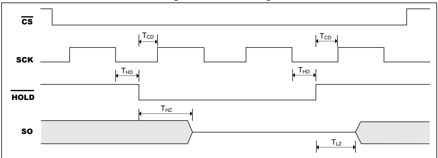
Figure 5-12. HOLD Timing
