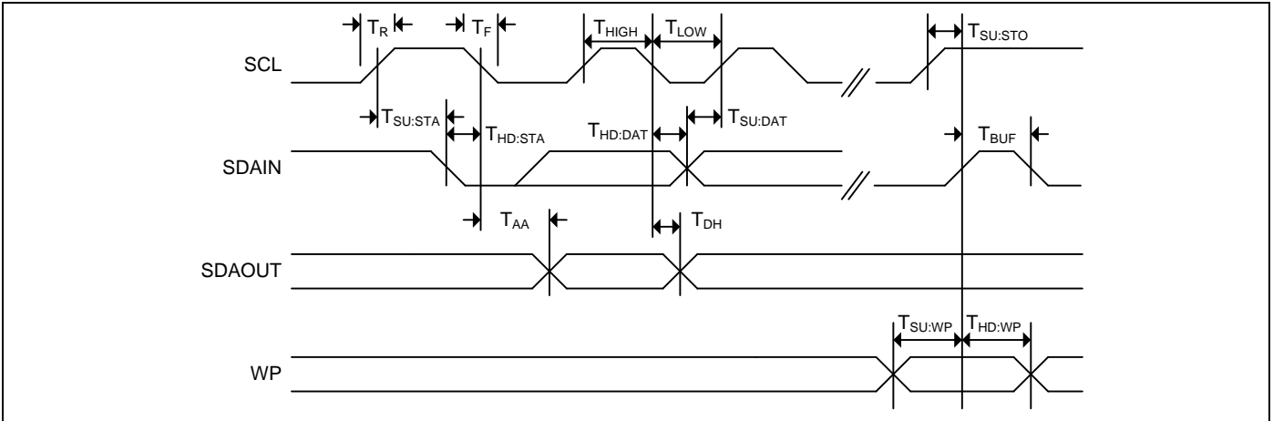
Figure 5-13. Bus Timing
