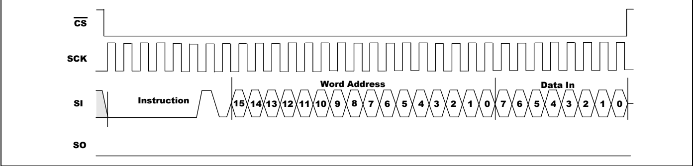
Figure 5-7. Write Timing
