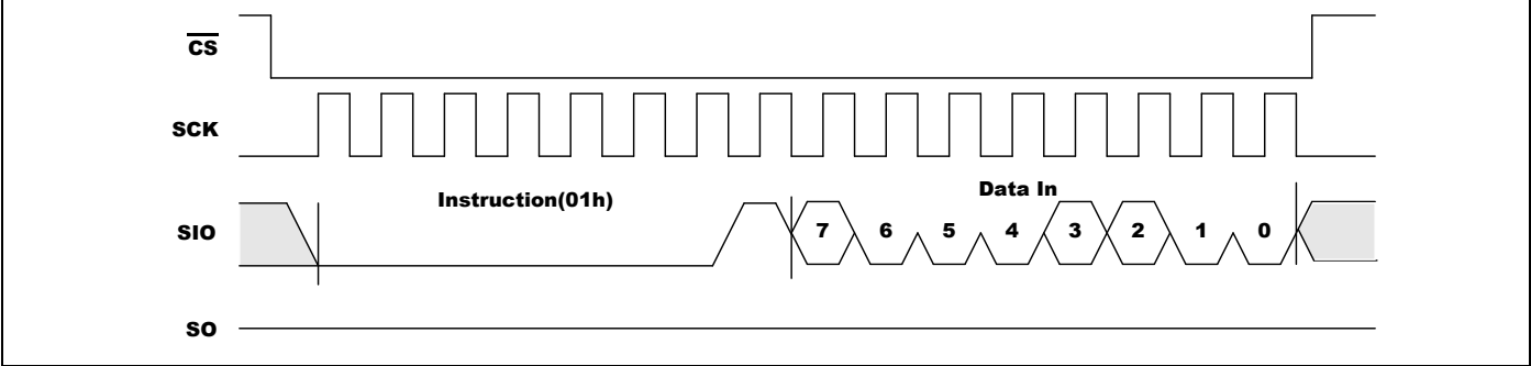
Figure 5-5. WRSR Timing
