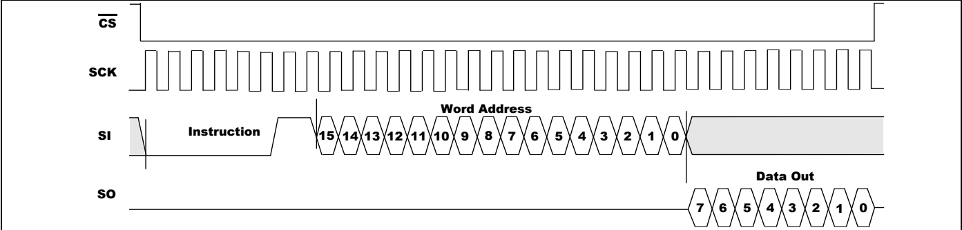
Figure 5-6. Read Timing
