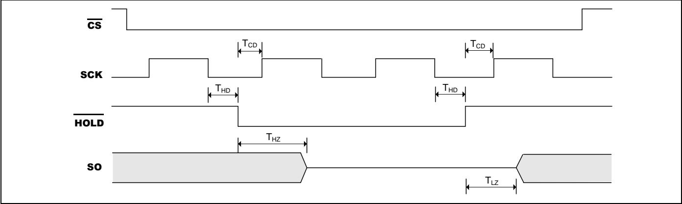
Figure 5-8. HOLD Timing
