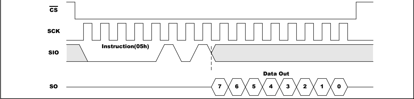
Figure 5-4. RDSR Timing
