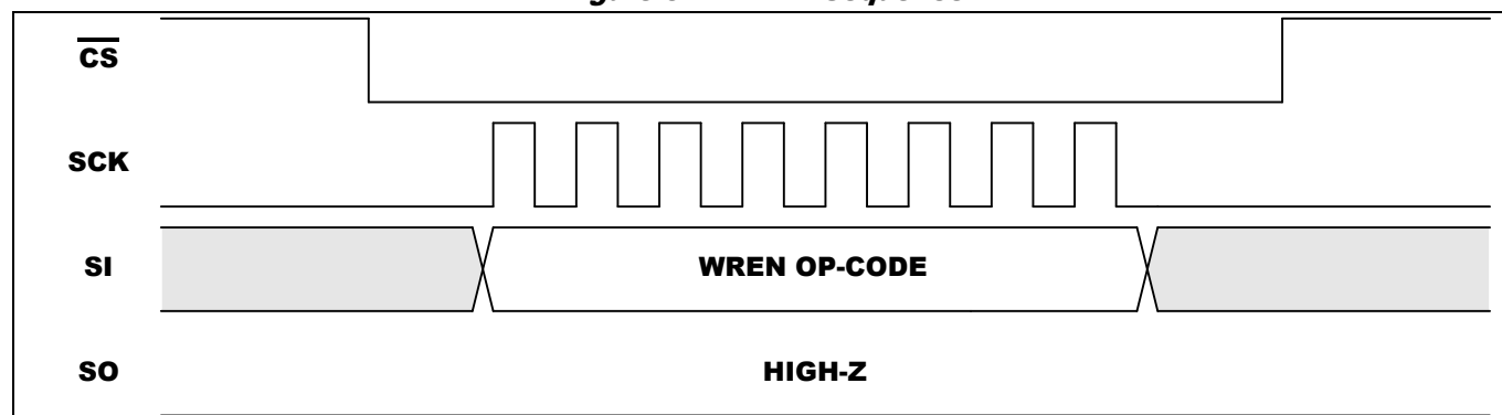
Figure 5-1. WREN Sequence
