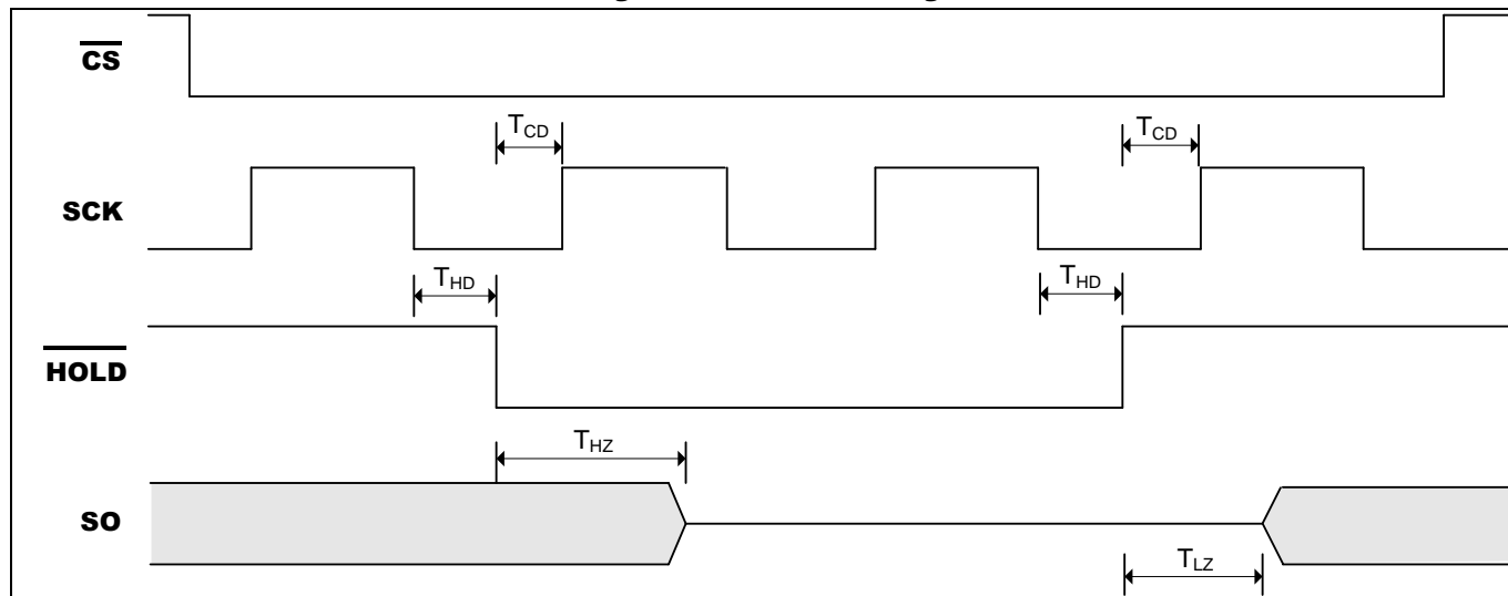
Figure 7-2. HOLD Timing
