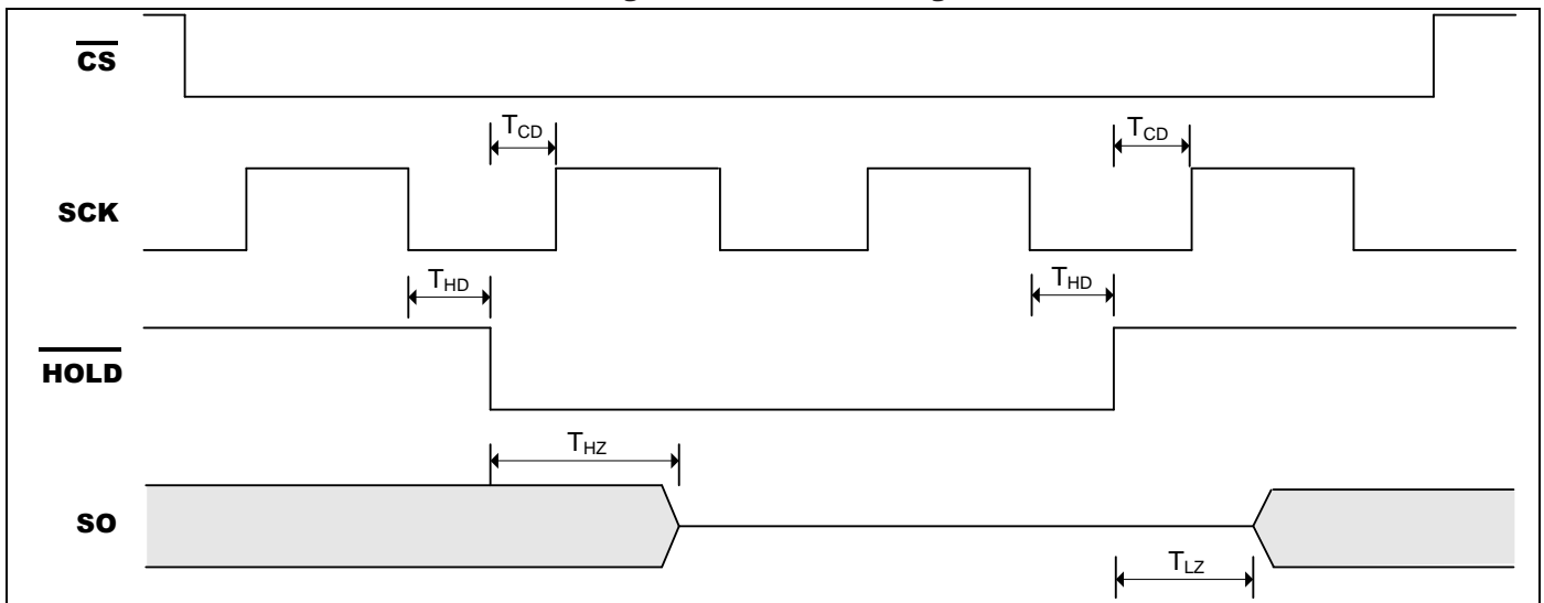
Figure 7-2. HOLD Timing
