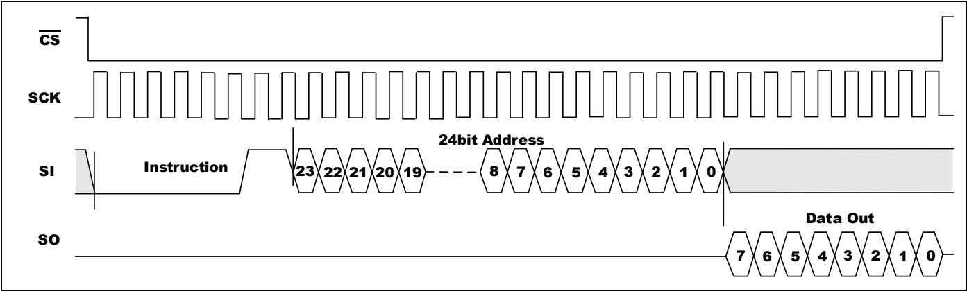
Figure 5-5. READ Sequence
