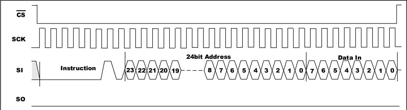
Figure 5-6. WRITE Sequence
