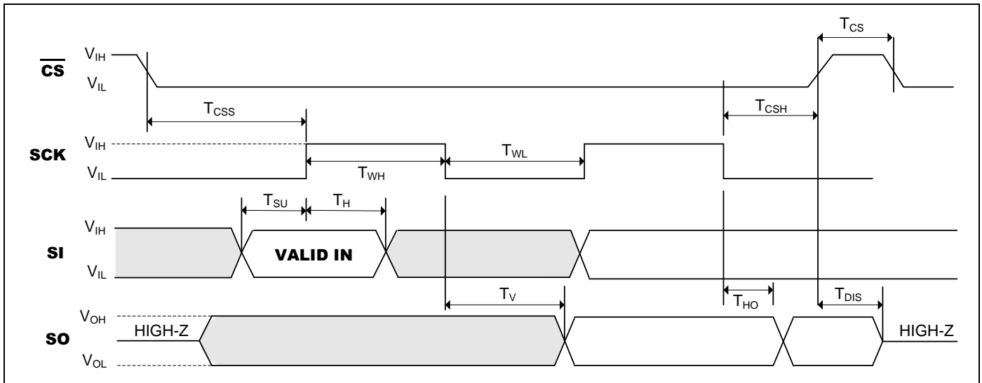
Figure 7-1. Synchronous Data Timing
