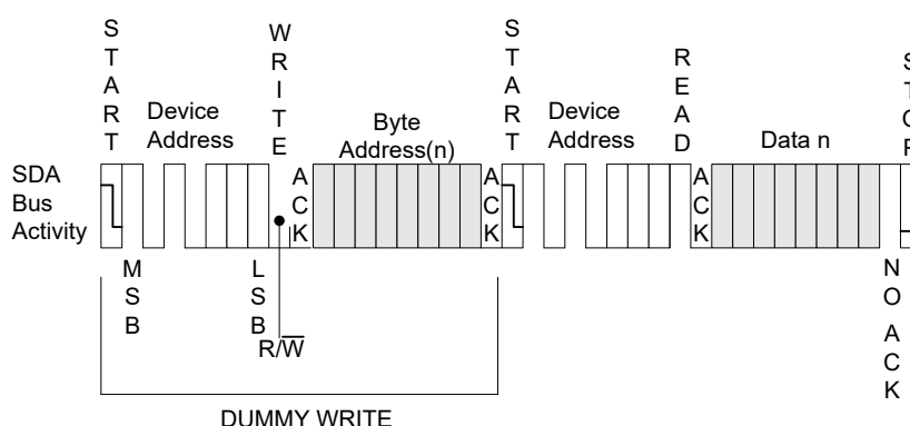
Figure 11. Random Address Read
