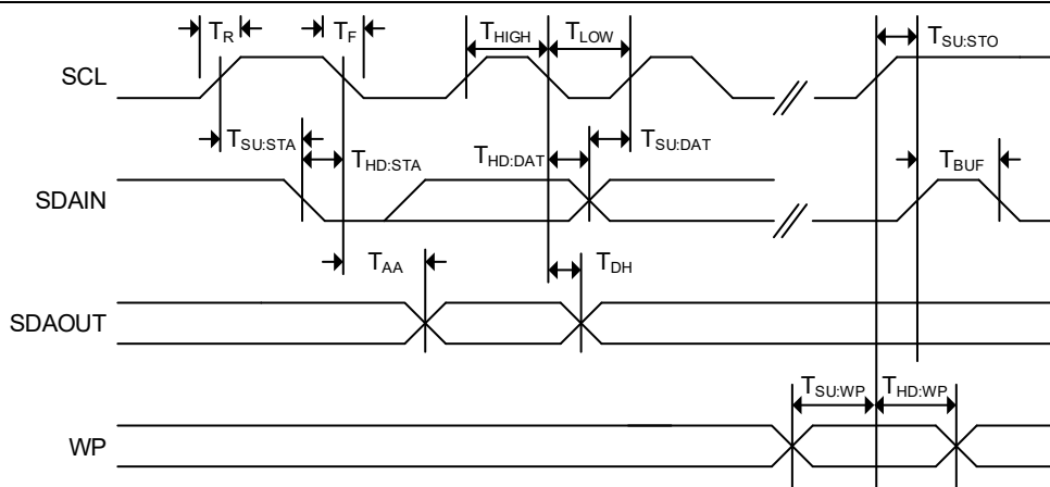
Figure 5-11. Bus Timing
