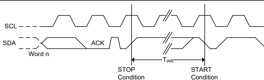
Figure 5-12. Write Cycle Timing
