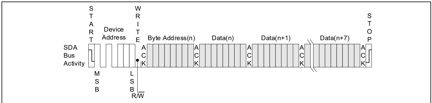
Figure 9. Page Write
