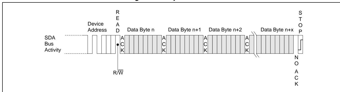
Figure 11. Sequential Read
