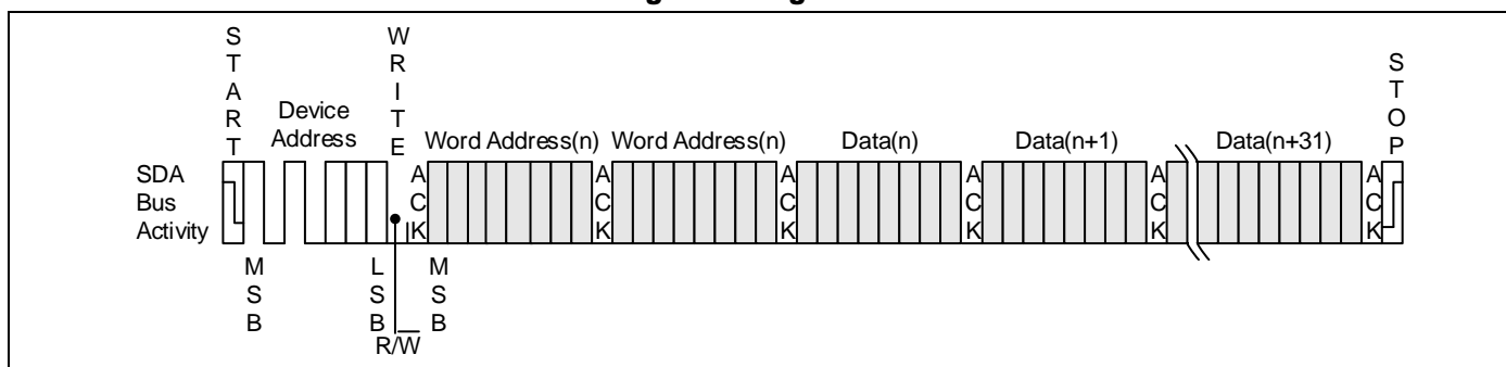
Figure 9. Page Write
