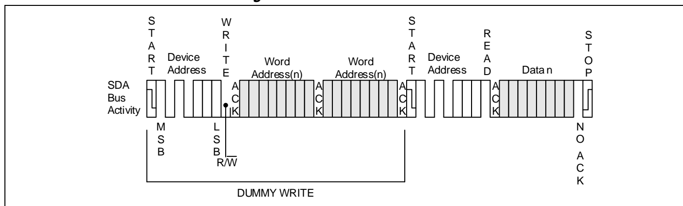
Figure 10 Random Address Read
