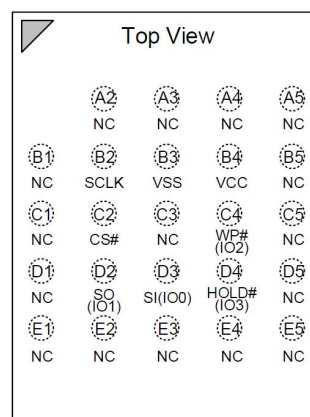
24-BALL TFBGA (5x5 ball array)
