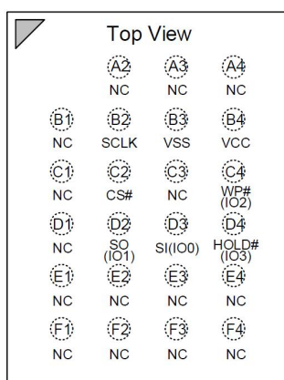
24-BALL TFBGA (6x4 ball array)
