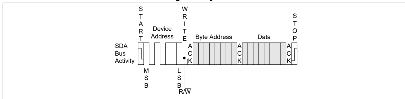
Figure 6. Byte Write
