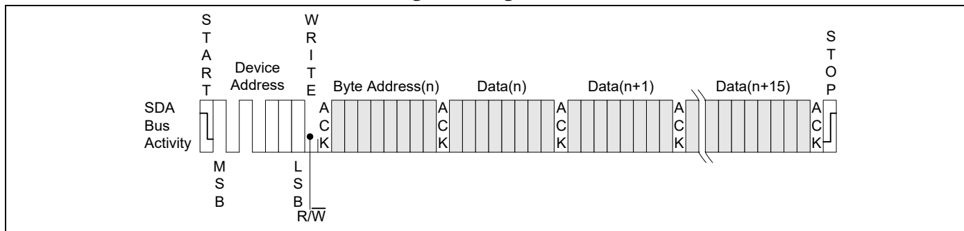
Figure 7. Page Write
