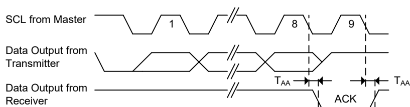
Figure 4. Output Acknowledge
