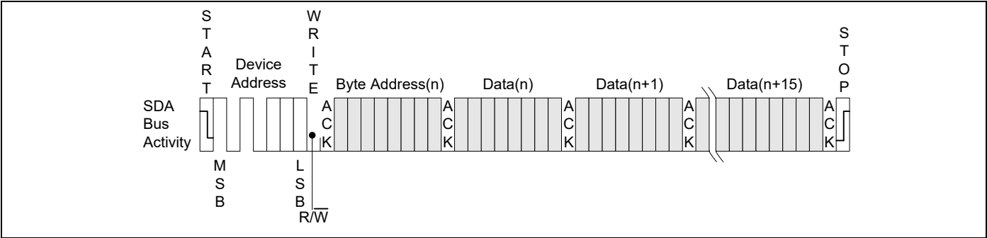
Figure 7. Page Write
