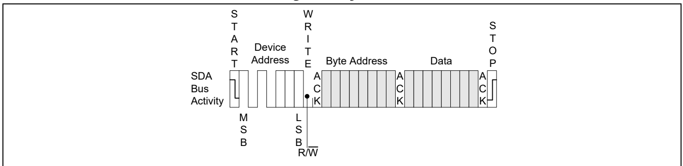
Figure 6. Byte Write
