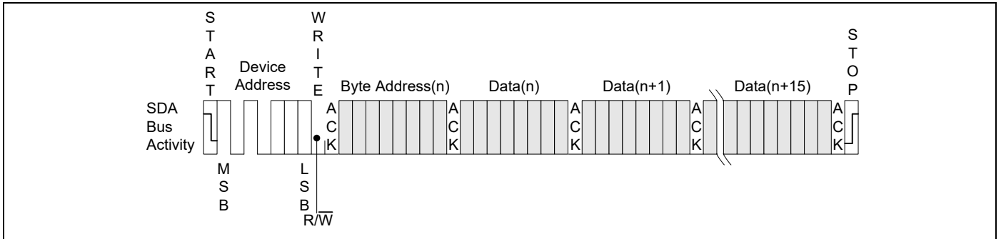
Figure 7. Page Write
