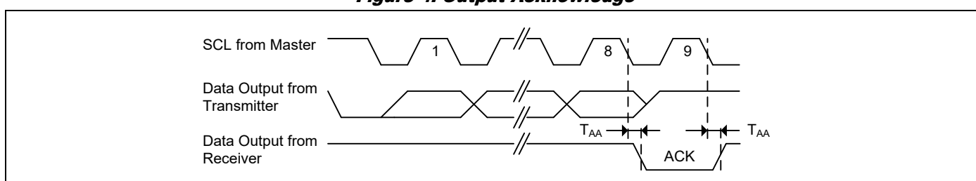
Figure 4. Output Acknowledge
