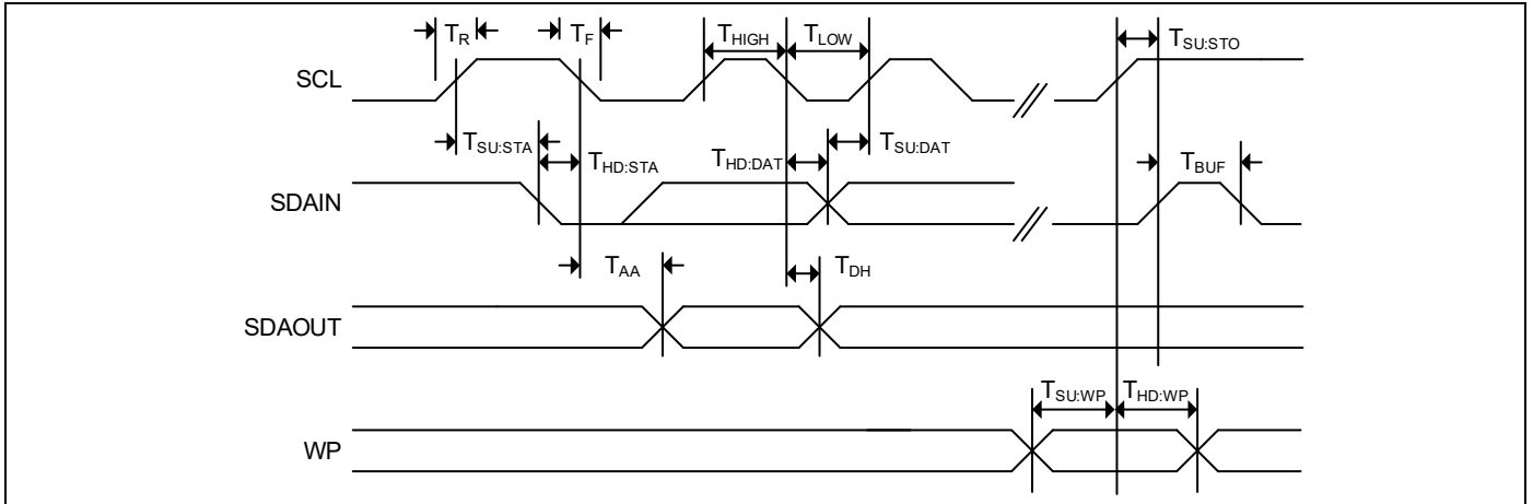
Figure 11. Bus Timing
