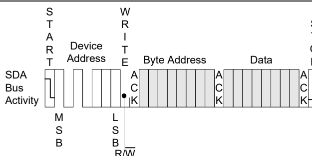
Figure 6. Byte Write
