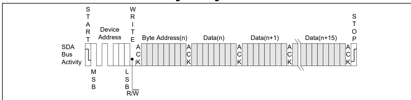
Figure 7. Page Write
