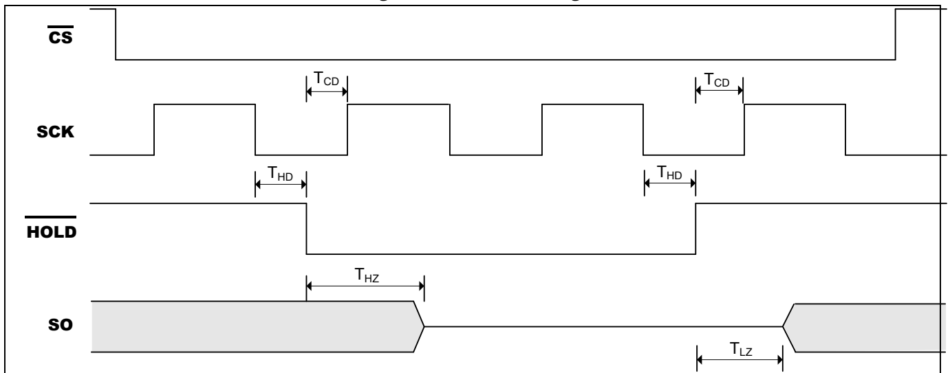
Figure 7-2. HOLD Timing
