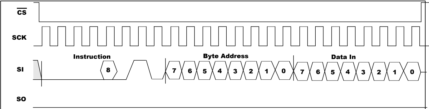
Figure 5-6. WRITE Sequence
