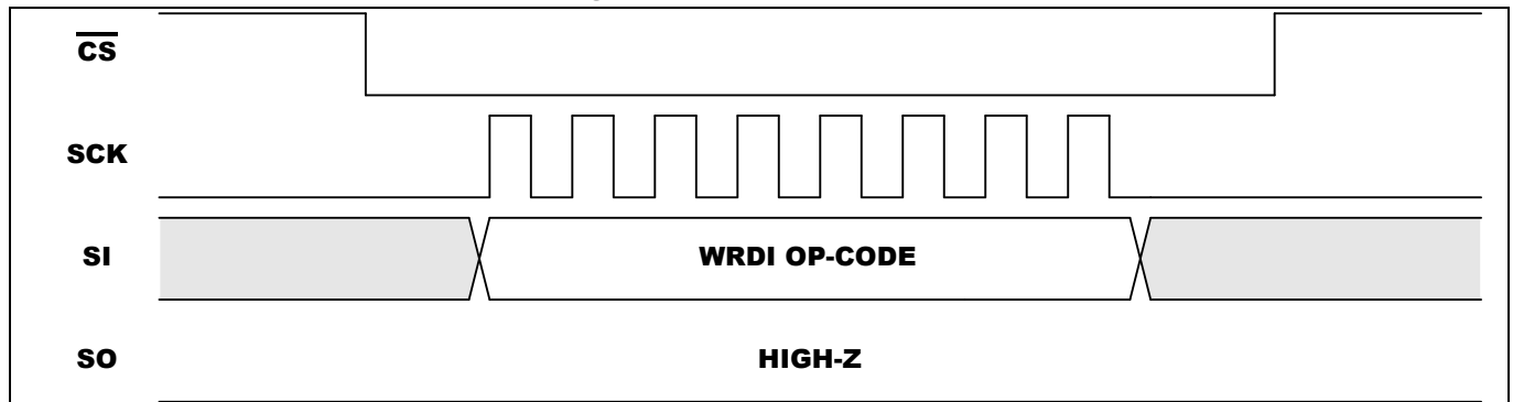
Figure 5-2. WRDI Sequence
