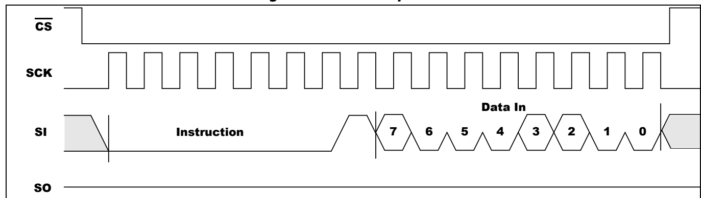
Figure 5-4. WRSR Sequence
