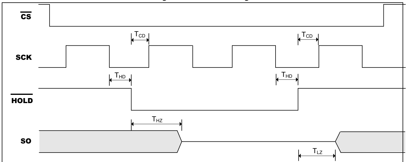
Figure 7-2. HOLD Timing
