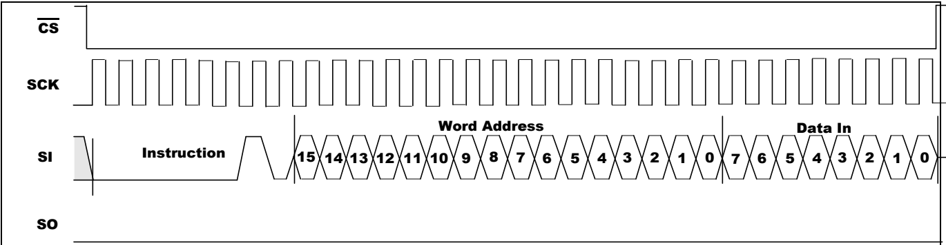
Figure 5-6. WRITE Sequence
