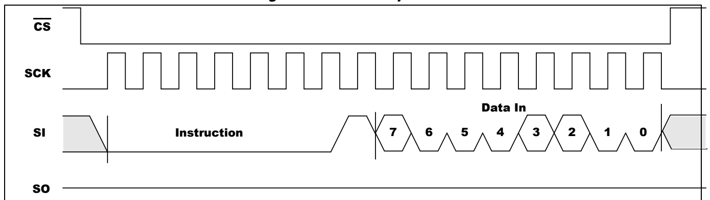
Figure 5-4. WRSR Sequence
