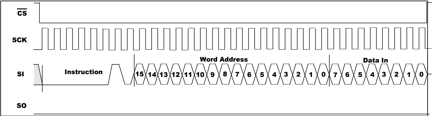
Figure 5-6. WRITE Sequence
