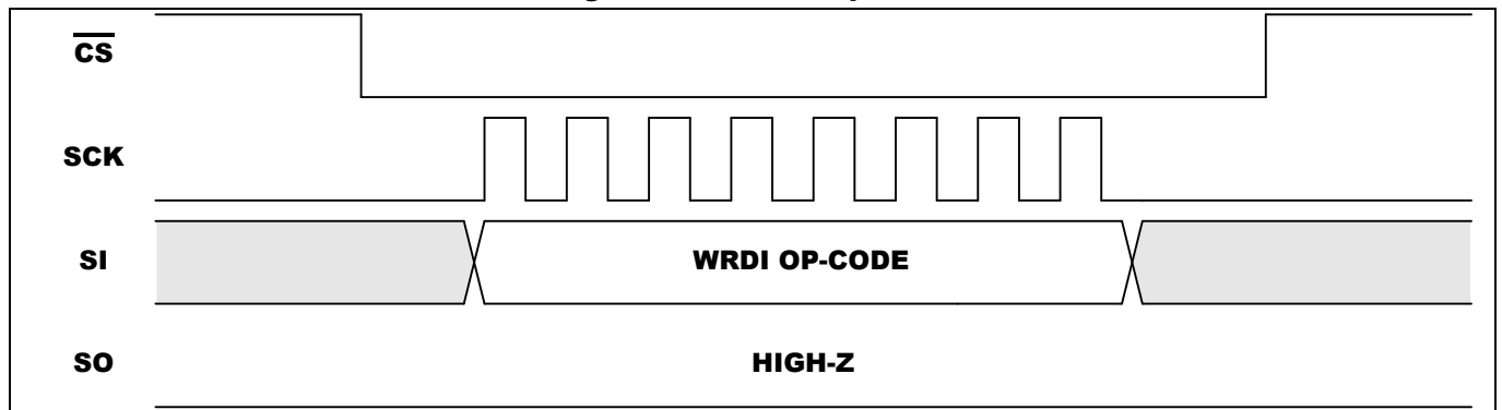
Figure 5-2. WRDI Sequence
