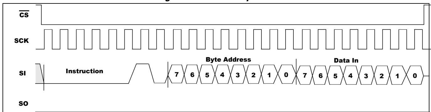
Figure 5-6. WRITE Sequence
