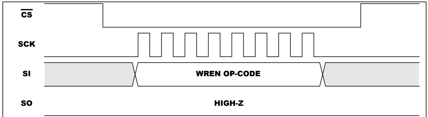
Figure 5-1. WREN Sequence
