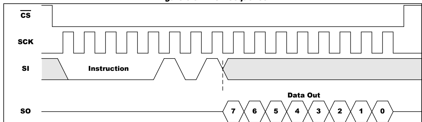
Figure 5-3. RDSR Sequence
