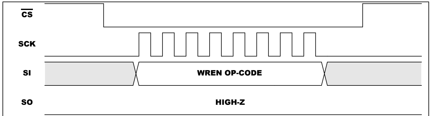
Figure 5-1. WREN Sequence
