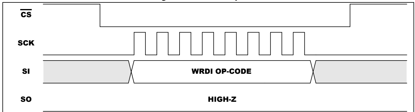
Figure 5-2. WRDI Sequence
