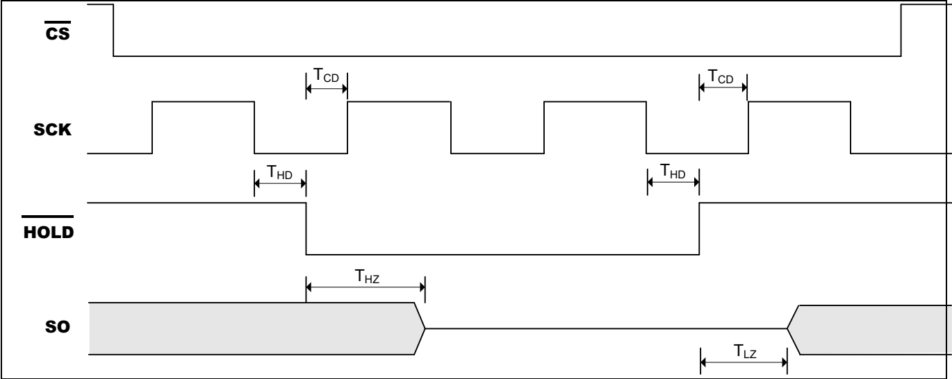
Figure 7-2. HOLD Timing
