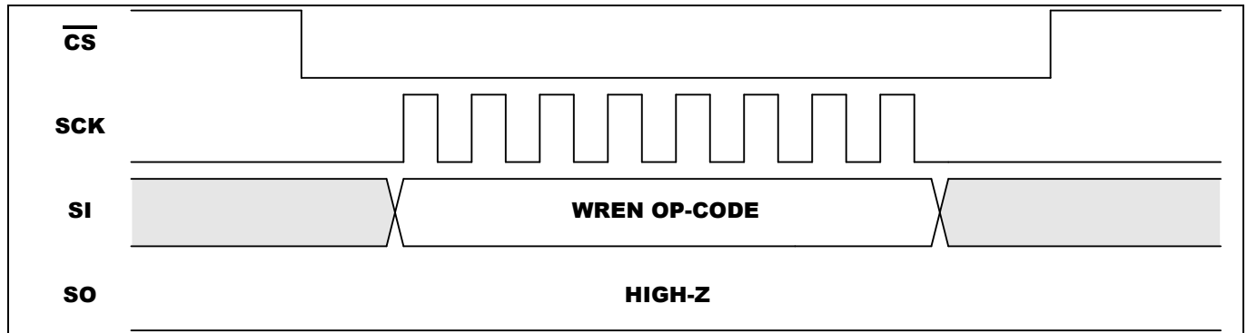
Figure 5-1. WREN Sequence
