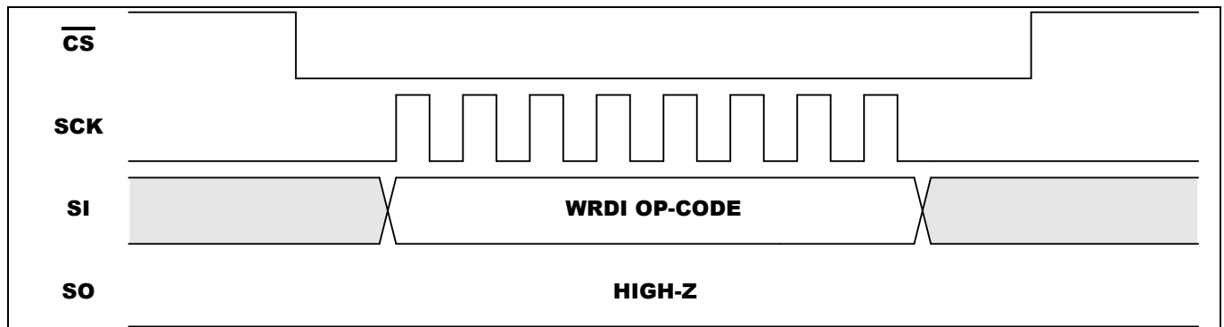
Figure 5-2. WRDI Sequence
