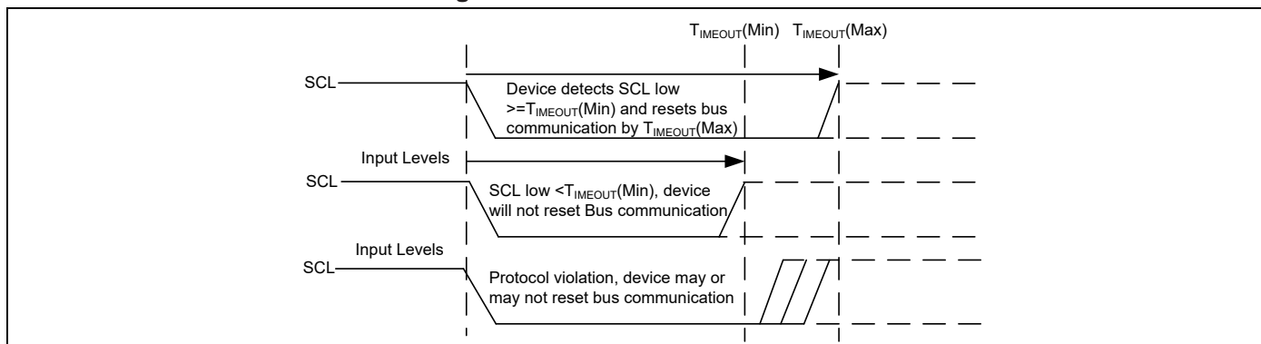
Figure 5.8. Bus Timeout Waveform
