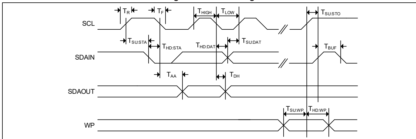
Figure 5.6. Bus Timing
