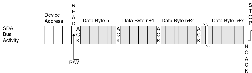
Figure 6.5 Sequential Read
