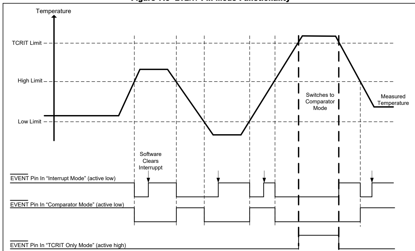
Figure 7.5 \overline{\text{EVENT}} Pin Mode Functionality
