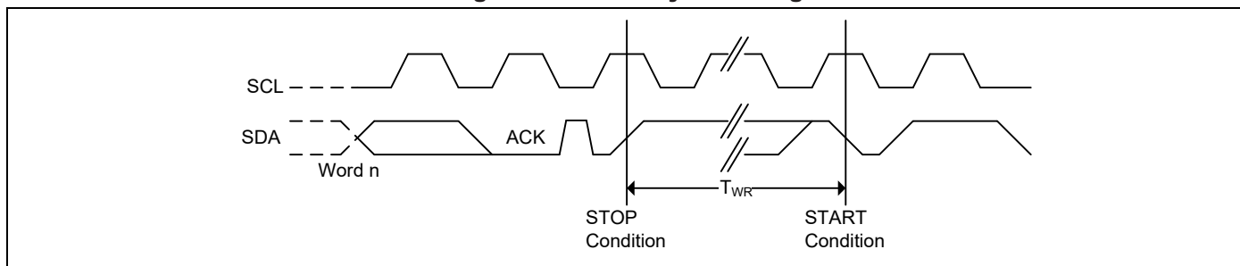
Figure 5.7. Write Cycle Timing
