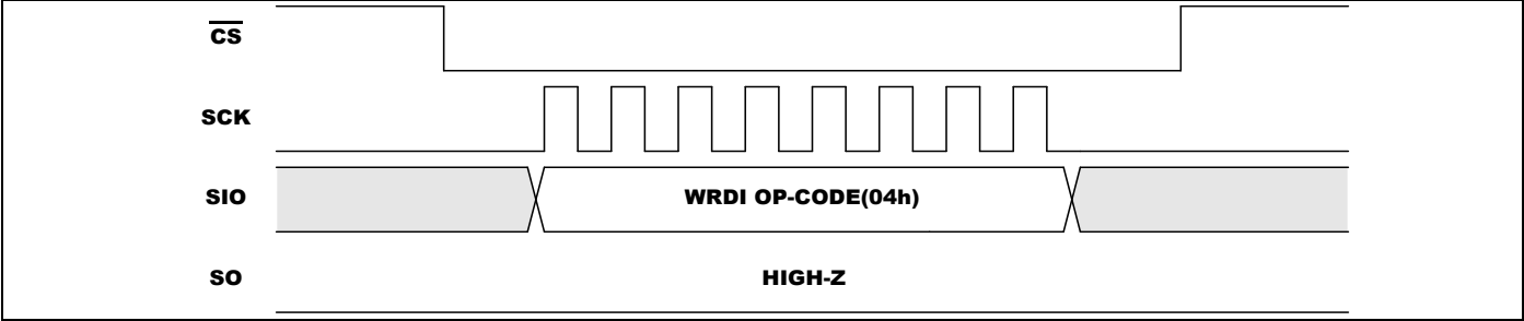
Figure 5-3. WRDI Timing
