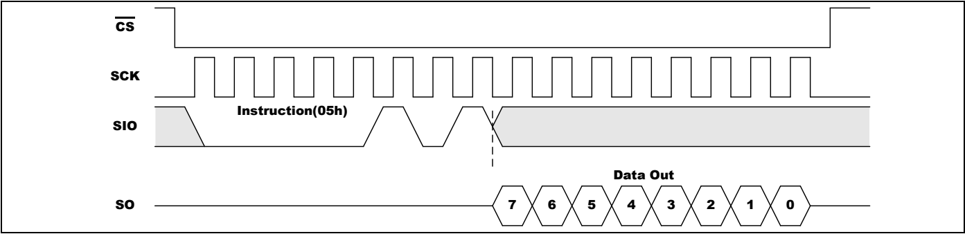
Figure 5-4. RDSR Timing
