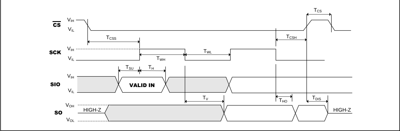
Figure 5-1. Synchronous Data Timing
