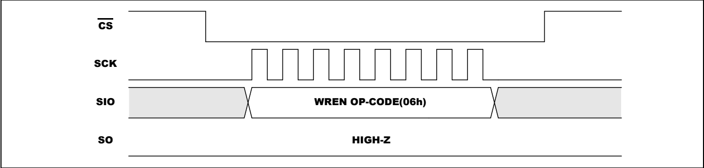
Figure 5-2. WREN Timing
