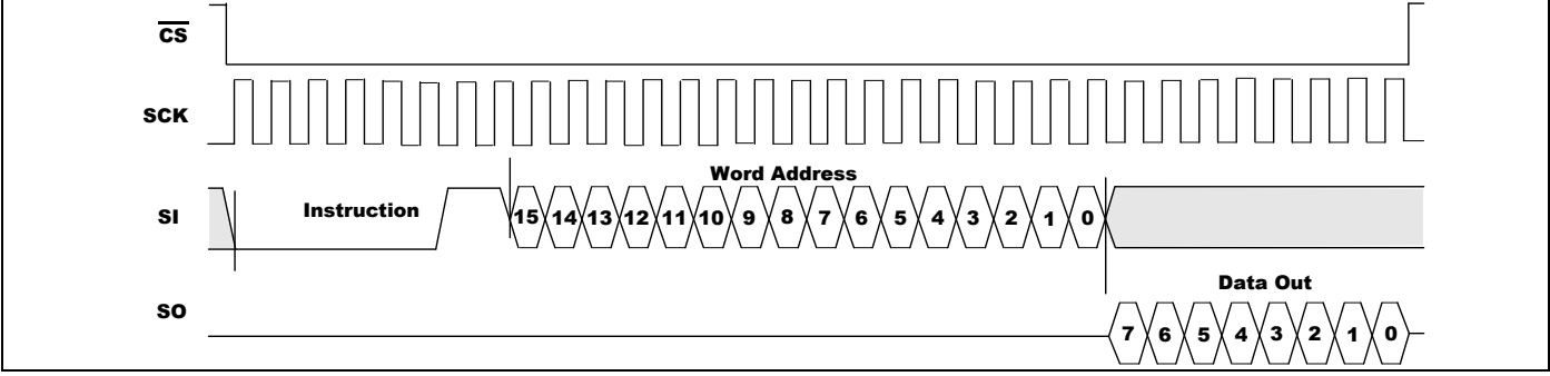
Figure 5-6. Read Timing
