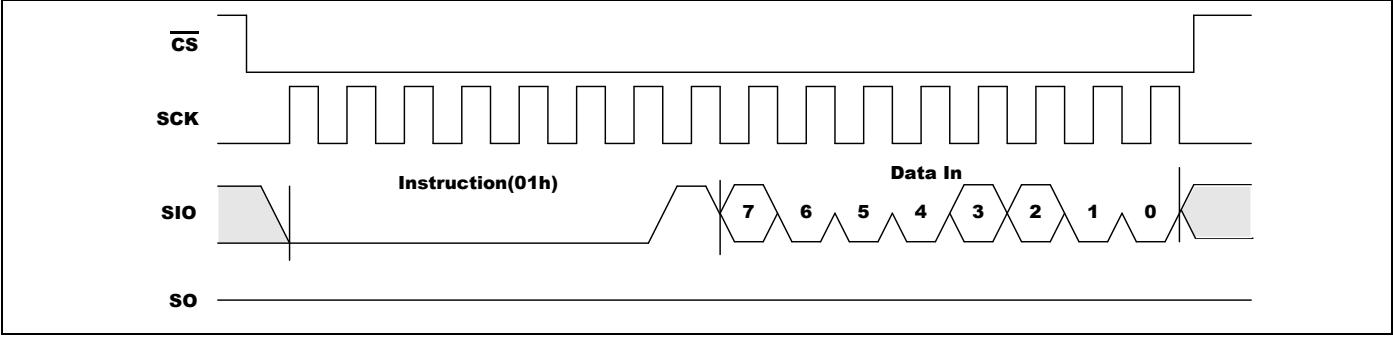
Figure 5-5. WRSR Timing
