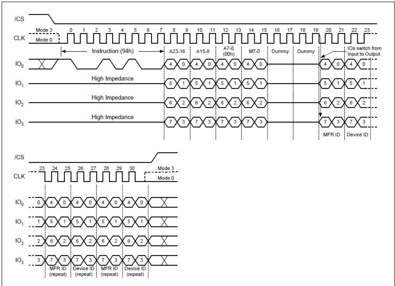
Figure24. Read Manufacture ID/ Device ID Quad I/O Sequence Diagram
