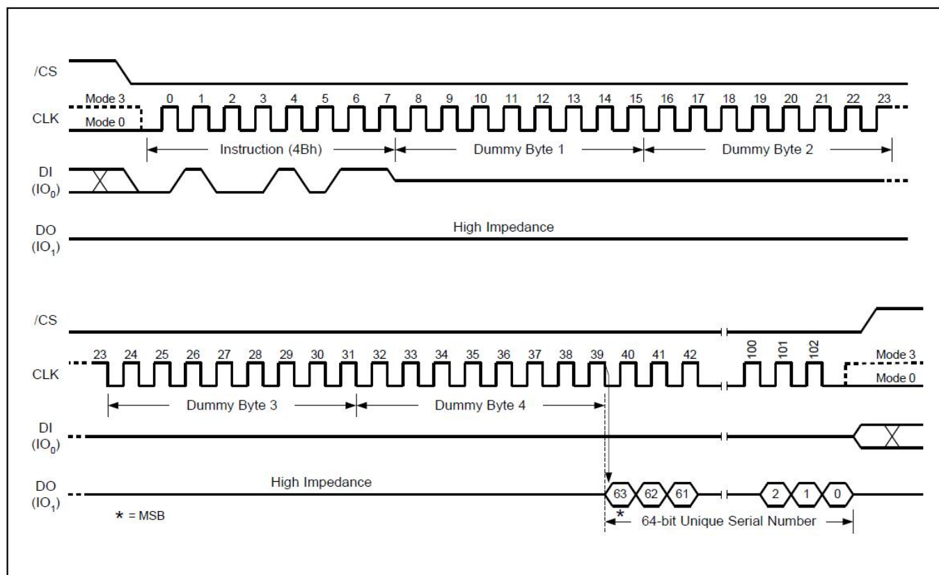
Figure26. Read Unique ID Number Instruction Sequence
