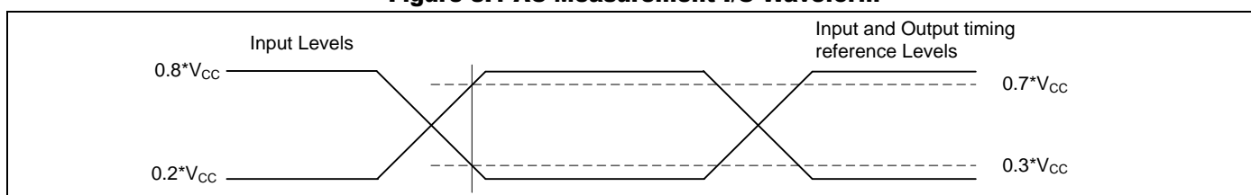
Figure 8.1 AC Measurement I/O Waveform
