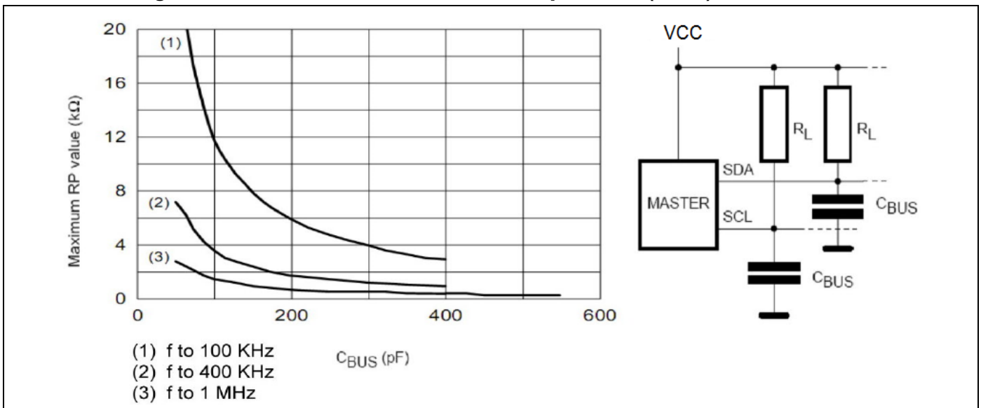
Figure 4.1 Maximum RL Value Versus Bus Capacitance (CBUS) for an I 2 C Bus
