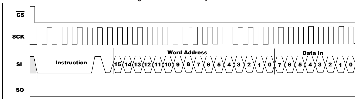
Figure 5-6. WRITE Sequence
